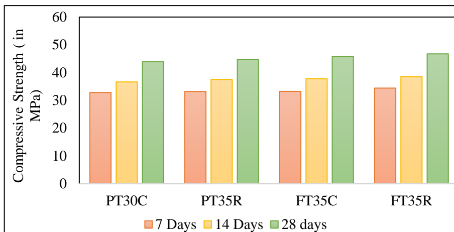
Figure 1. Compressive Strength for M30
