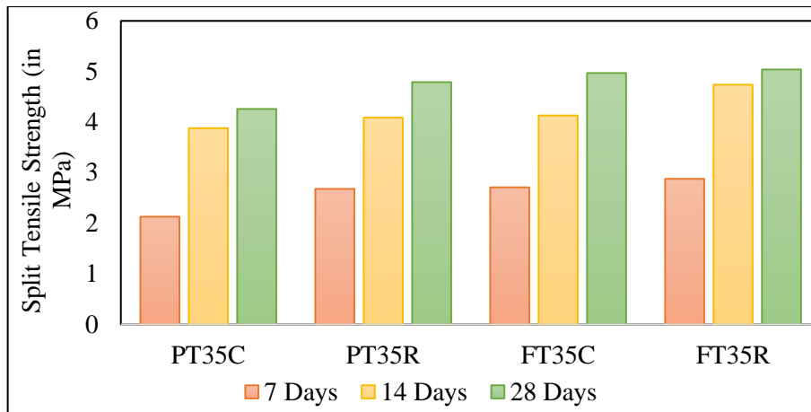
Figure 4. Split Tensile Strength for M35
