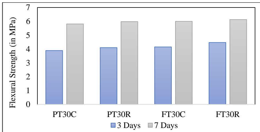
Figure 5. Flexural Strength for M30
