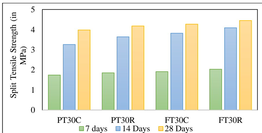
Figure 3. Split Tensile Strength for M30
