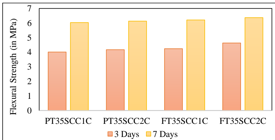
Figure 6. Flexural Strength for M35
